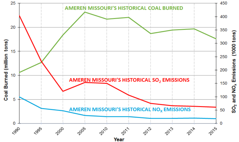
Ameren Missouri Coal-Fired Generation Historical Coal Burned, Nitrogen Oxide and Sulfur Dioxide Emissions
